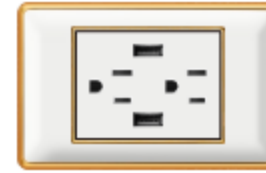
C3-024 Duplex Socket+USB 10-16A 110-250V 50/60Hz 5V 2100mA
